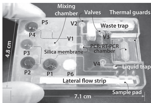
Fig. 2: Disposable cartridge for PCR.
